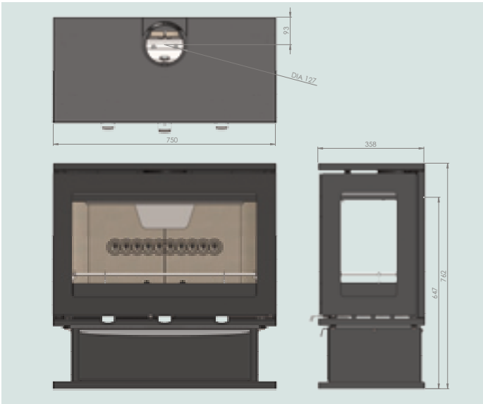
LPV8 on Pedestal Stand
