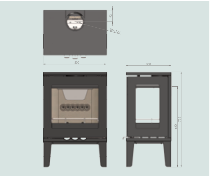
LPV5 on Leg Stand
