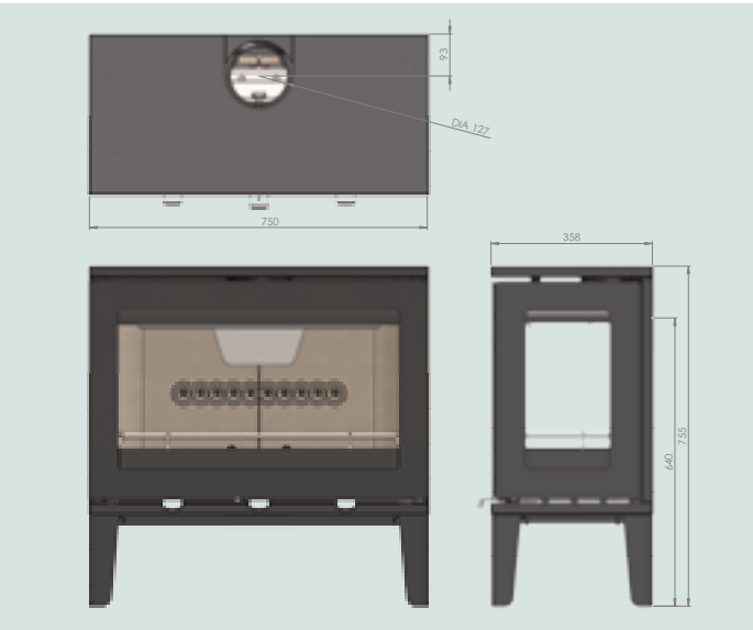
LPV8 on Leg Stand
